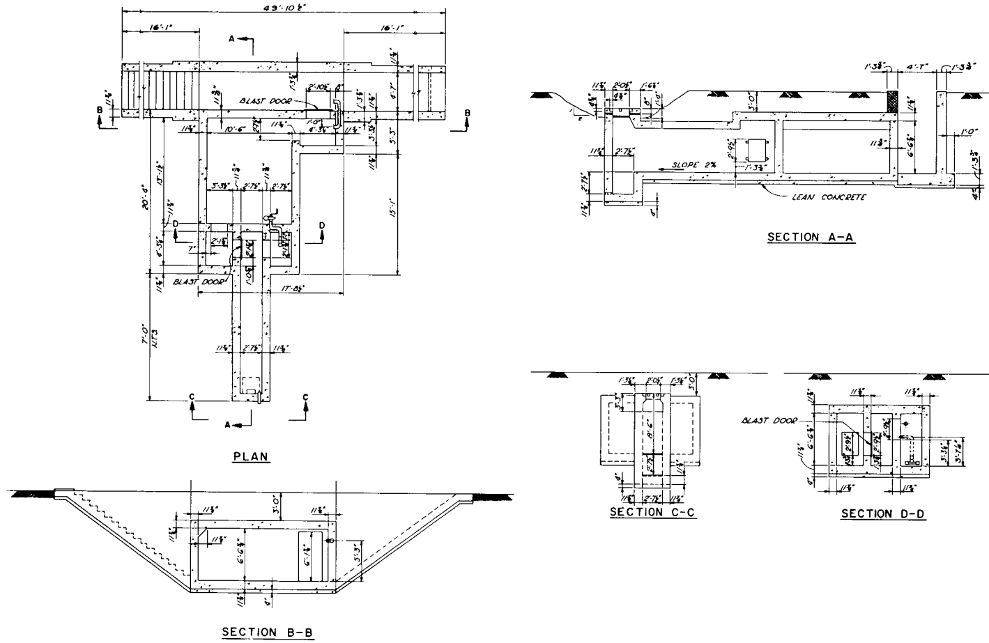
Fig. 4—Architectural layout for type-C rectangular shelter.
